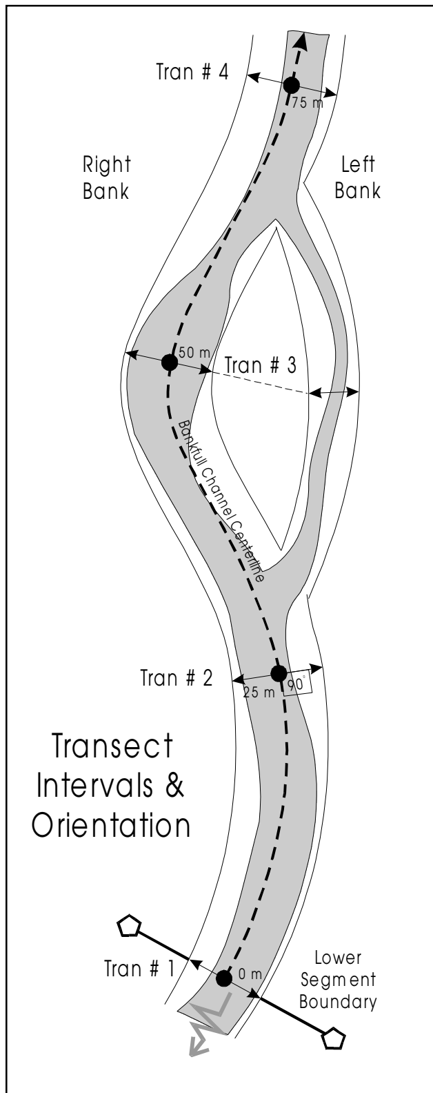
Figure 4. Transect intervals are measured along the center line of the bankfull channel.
