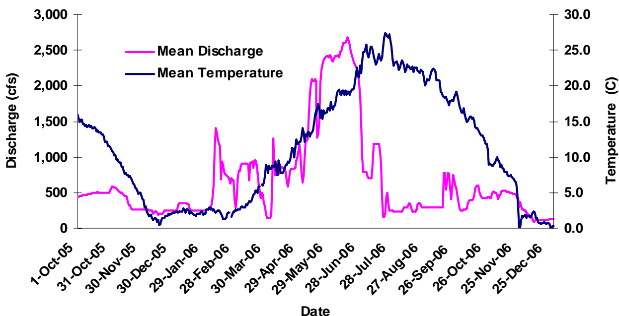
Figure 9. Daily mean temperature and discharge for the Okanogan River below Zosel Dam from 1 October 2005 through 31 December 2006. Data are from the USGS gauge at Oroville, WA ( http://waterdata.usgs.gov/wa/nwis ).
