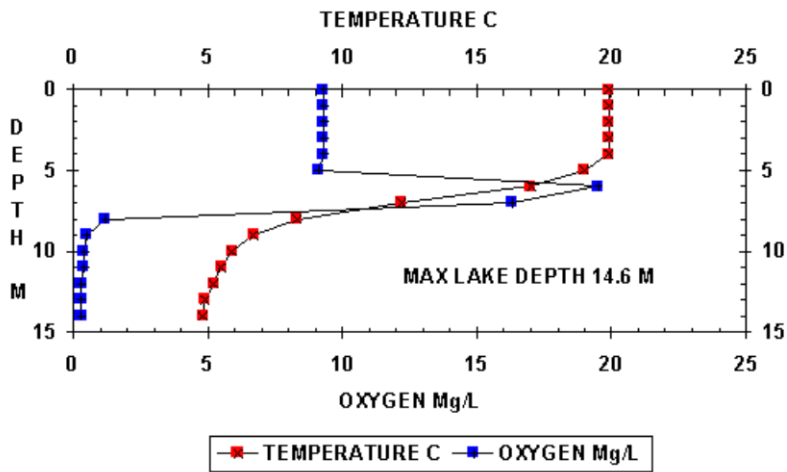
OXYGEN-TEMPERATURE PROFILE FOR NORTH TWIN LAKE 18 SEPTEMBER 1998
