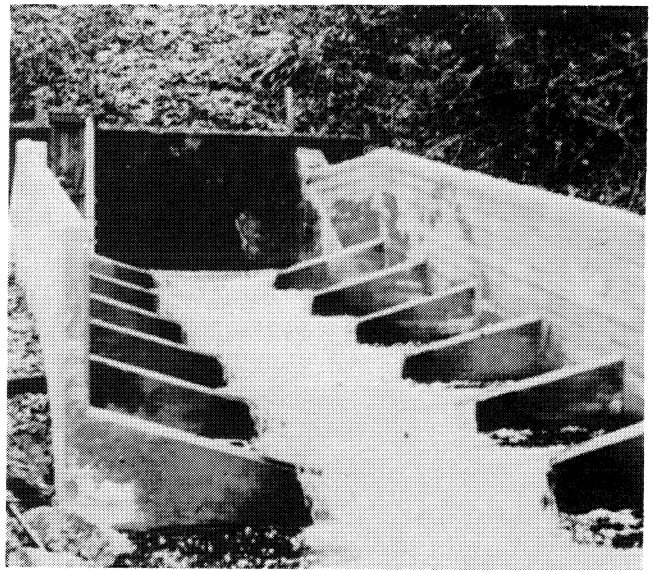
PHOTO 05-7. Modified pool and weir fishway provides access through a culvert on Harvey Creek.
