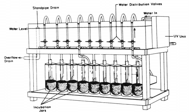
Fig. 83. Diagram of a sturgeon hatchery system using modified MacDonald jars. UV = ultraviolet treatment (Monaco and Doroshov 1983)
