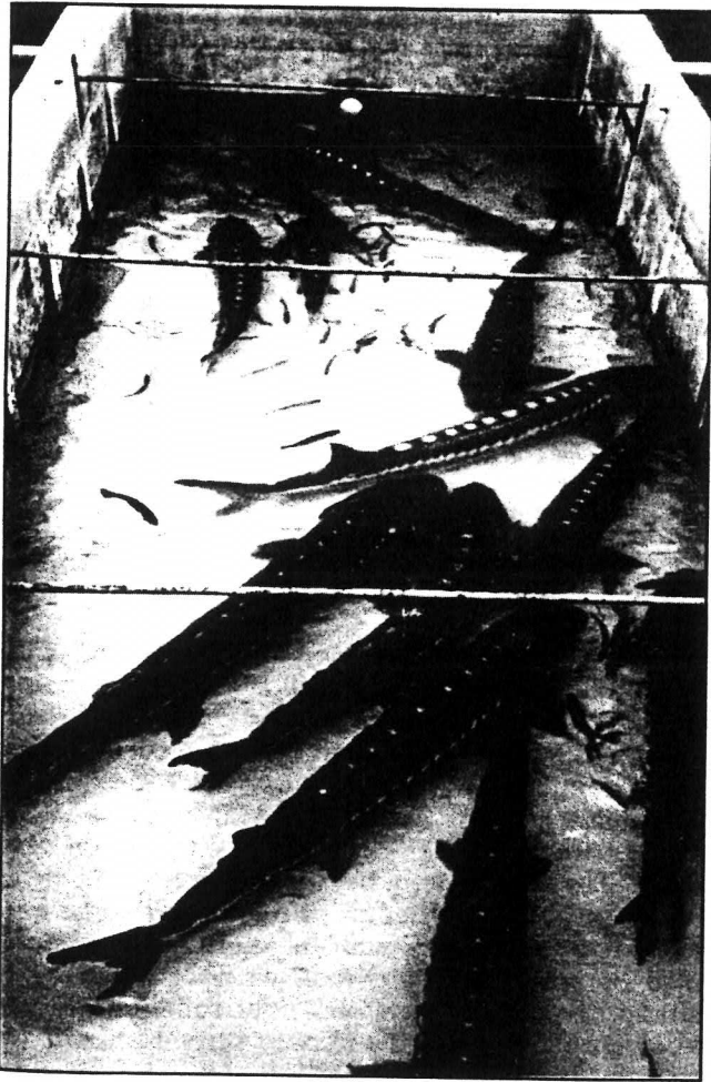
Fig. 44. Fiberglass acclimation tank for sturgeon captured in salt water.
