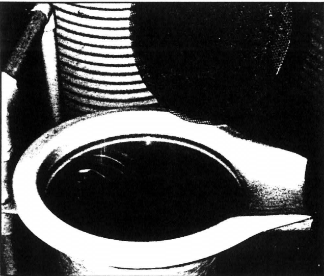
Fig. 88. A 3.0-mm mesh screen used to cap the modified trout egg barrel and prevent sturgeon eggs from flowing out with the discharge water.
