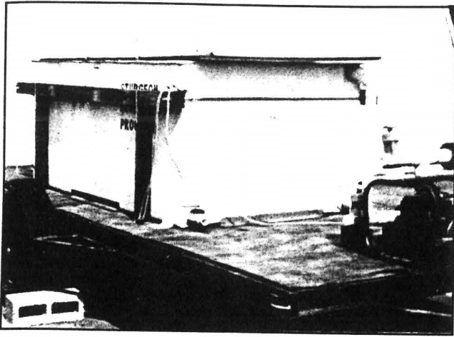
Fig. 43. Insulated fiberglass transport tank for sturgeon broodstock mounted on a double-axle trailer and equipped with a water circulation system and supplementary aeration.
