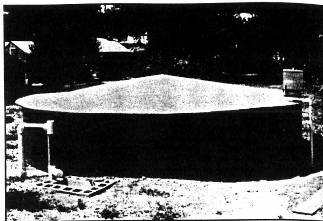
Fig. 45. Six-meter diameter fiberglass tank with peaked fiberglass sectional roof used for long-term holding and as maturation tanks for sturgeon broodstock.
