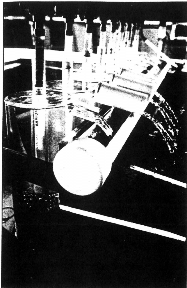
Fig. 92. A sturgeon hatchery system showing the use of extension tubes to direct water flow from the hatchery jars to the water recirculation system, the larval collecting tank, or a silt sump.
