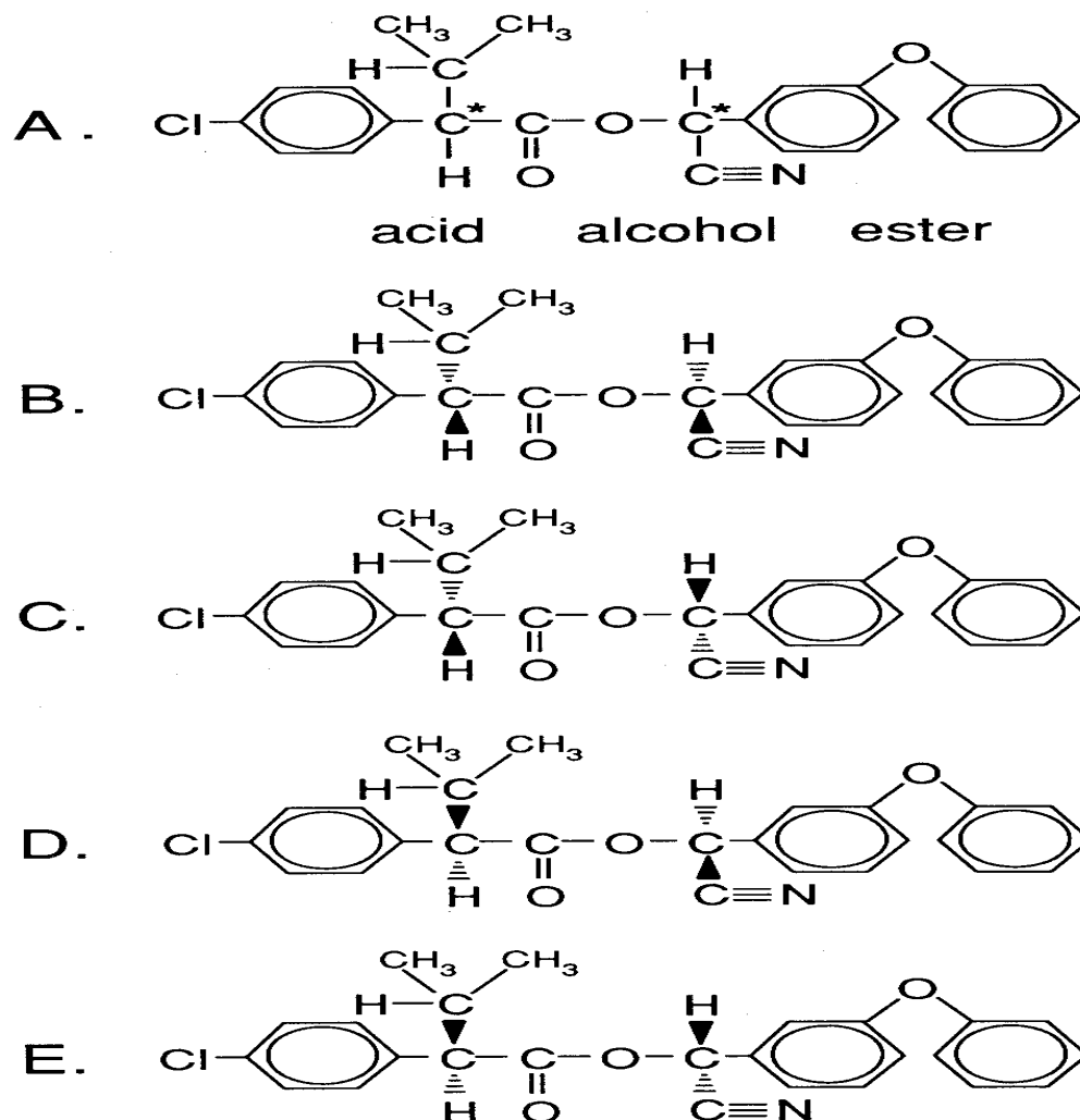
Figure. Fenvalerate and its isomers (Ohkawa et al. 1979; Hill 1981; Kaneko et al. 1981, 1986; Vijverberg and Bercken 1982; Miyamoto et al. 1986; Bradbury et al. 1987b; Bradbury and Coats 1989a, 1989b; Coats et al. 1989).
